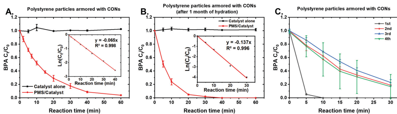
Fig. 5 Catalytic oxidation of BPA by PMS under activation by (A) fresh CON-armed polystyrene particles, (B) CON-armed polystyrene particles after 1 month of hydration, and (C) fresh CON-armed polystyrene particles upon repeated use. Experimental conditions: [\text{PMS}]_0 = 500 \mu\text{M} ; [\text{BPA}]_0 = 5 \mu\text{M} ; [\text{catalyst}] = 0.04 \text{ g L}^{-1} ; pH = 5 with 0.02 M acetate buffer. Error bars stand for data ranges of experimental replicates ( n \geq 2 ).
