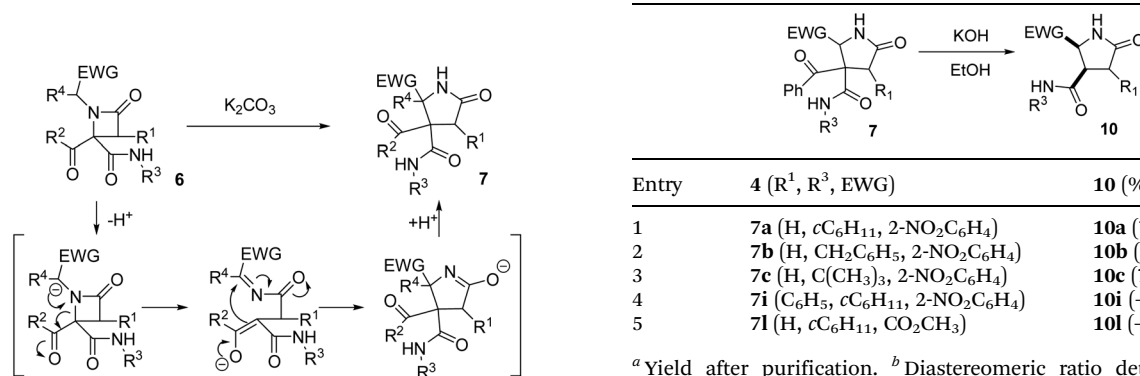
Scheme 2 Proposed mechanism for the anionic rearrangement from azetidines 6 to pyrrolidinones 7 .
