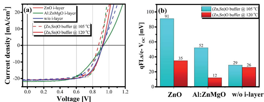
Fig. 2 (a) The characteristic J - V curves of the \text{Cu(In,Ga)S}_2 devices prepared with (\text{Zn,Sn})\text{O} buffer layers deposited at 105^\circ\text{C} (B1) and 120^\circ\text{C} (B2), represented by dashed and solid lines respectively. The devices prepared with ZnO, Al:ZnMgO and without an i-layer are represented by red, green and blue lines, respectively. (b) Interface V_{\text{OC}} deficit bar plot of devices made with B1 and B2 with various i-layer combinations.
