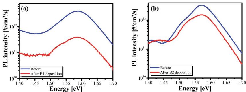
Fig. 1 (a) Absolute calibrated photoluminescence spectra of \text{Cu(In,Ga)S}_2 before and after (\text{Zn,Sn})\text{O} buffer layer was deposited at (a) 105^\circ\text{C} (B1) and (b) 120^\circ\text{C} (B2), measured at an illumination intensity equivalent to one sun.
