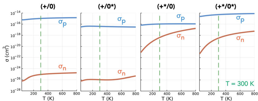
Fig. 6 Electron and hole capture cross-section ( \sigma_n and \sigma_p ) as functions of temperature T for the \text{Te}_i (+^*/0^*) charge transition levels in CdTe. Room temperature ( T = 300 K) denoted by the dashed green line as a guide for typical solar cell operating conditions.
