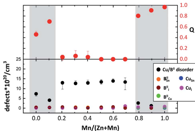
Fig. 8 Concentration of \text{Cu}_{2d} and \text{B}_{2c}^{\text{II}} point defects (related to \text{Cu}/\text{B}^{\text{II}} disorder) and \text{Cu}_{\text{Snr}} , \text{Cu}_i , \text{I}_{\text{Cu}} , \text{I}_{\text{Sn}} and \text{I}_i point defects (related to the off-stoichiometry type), as well as the order parameter Q calculated from the Cu and \text{B}^{\text{II}} distribution on the Wyckoff positions 2c and 2d (according to eqn (5)) dependent on the Mn/(Mn + Zn) ratio.
