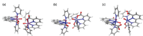
Fig. 7 Transition state structures of [Ru V (bda)(py) 2 -O] + dimer (a, O–O distance 1.9 Å), [Fe V (bda)(py) 2 -O] + dimer (b, O–O distance 2.1 Å) and 6-coordinate [Fe V (bda)(py) 2 -O] + dimer (c, O–O distance 2.0 Å).
