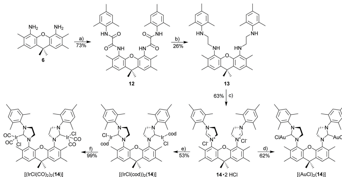
Scheme 5 Synthesis of imidazolium salt 14·2HCl and derived metal complexes. Reagents and conditions: (a) \text{MesNHC(O)COCl} , \text{NEt}_3 , 0 °C to rt, 1 h; (b) \text{BH}_3 \cdot \text{THF} , reflux, 3 d; (c) triethyl orthoformate, \text{NH}_4\text{Cl} , 110 °C, 24 h; (d) [\text{AuCl}(\text{SMe}_2)] , \text{K}_2\text{CO}_3 , acetone/ \text{CH}_2\text{Cl}_2 , 50 °C; (e) [\text{IrCl}(\text{cod})]_2 , \text{K}_2\text{CO}_3 , acetone/ \text{CH}_2\text{Cl}_2 , 50 °C; (f) CO, 0 °C, 30 min, \text{CH}_2\text{Cl}_2 .
