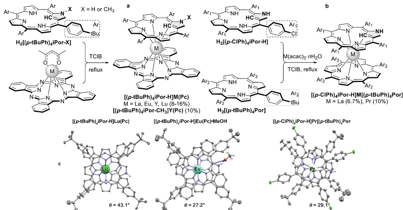
Scheme 31 (a and b) Synthesis of heteroligand double-decker complexes with N-confused ligands. (c) X-ray structures of [(\text{p-tBuPh})_4\text{iPorH}]\text{Lu}(\text{Pc}) (CCDC YEFZIU), [(\text{p-tBuPh})_4\text{iPorH}]\text{Eu}(\text{Pc})\cdot\text{MeOH} (CCDC YEFZAM) 171 and [(\text{p-ClPh})_4\text{iPorH}]\text{Pr}[(\text{p-tBuPh})_4\text{Por}] (CCDC BODFIL). 172 Solvate molecules and most of hydrogen atoms are not shown for clarity.
