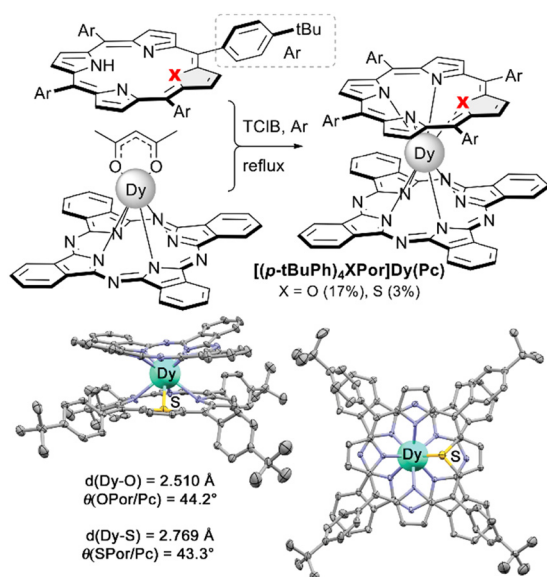
Scheme 32 Synthesis of mixed ligand double-decker complexes with oxa- and thiaphthalocyanine ligands and X-ray structure of [(\text{p-tBuPh})_4\text{SPor}]\text{Dy}(\text{Pc}) (CCDC AHOPUK). 173 Hydrogen atoms and solvent molecules are not shown for clarity.
