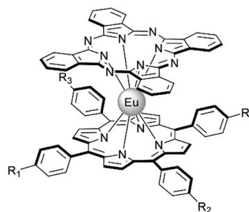
Fig. 6 Amino-substituted mixed ligand complexes ( (\text{A}_1\text{-TPP})Eu(\text{Pc}) : R_1 = \text{NHOct} , R_2 = R_3 = \text{H} ; ( \text{A}_2\text{-TPP})Eu(\text{Pc}) : R_1 = R_2 = \text{NHOct} , R_3 = \text{H} ; ( \text{A}_4\text{-TPP})Eu(\text{Pc}) : R_1 = R_2 = R_3 = \text{NHOct} ). 133,134
