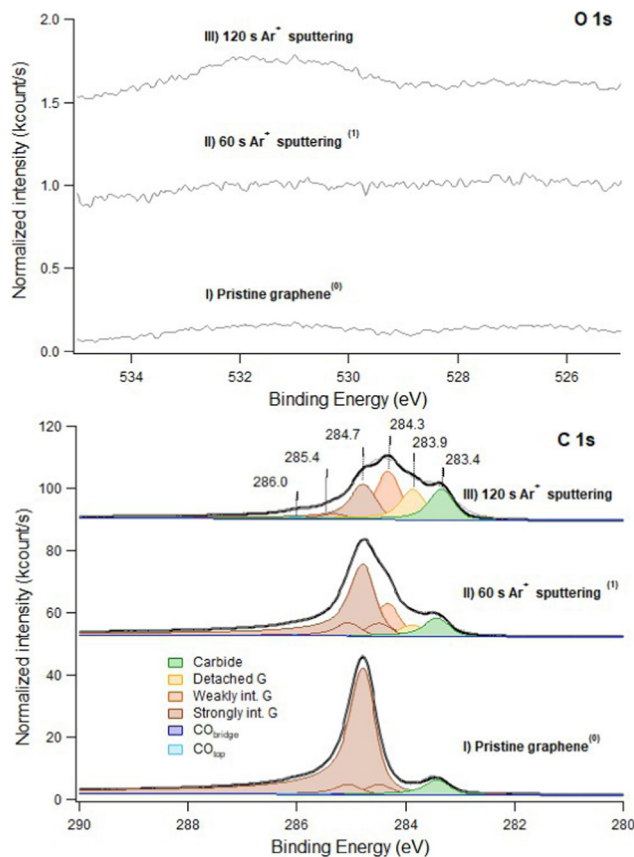
Fig. 1 C 1s (bottom panel) and O 1s (top panel) spectra recorded at h\nu 650 eV. Trace I: pristine layer, recorded immediately after graphene growth. Trace II: defected layer obtained after 60 s sputtering with \text{Ar}^+ ions (kinetic energy of 150 eV; Ar pressure of 1 \times 10^{-5} mbar). Trace III: same as II after 120 s sputtering in identical conditions. Only very weak signals are present in the O 1s spectrum (note the difference in the intensity scale between the C 1s and O 1s regions). This indicates that no extended Ni areas are exposed to the residual gas since they would be promptly covered by CO. The apex numbers appearing after the description of the spectra refer to their position in the sequence reported in Fig. 6.
