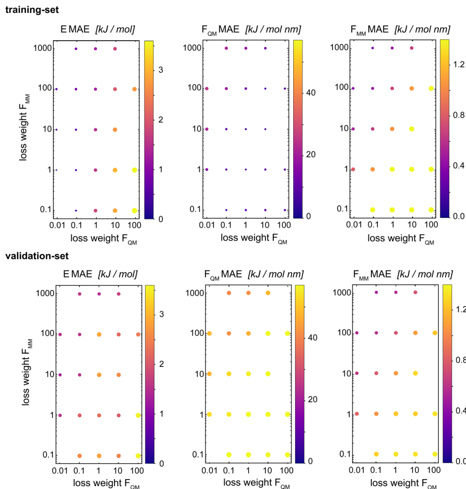
Fig. 5 Influence of relative weights ( wF_{\text{QM}} and wF_{\text{MM}} ) for the different loss terms (QM forces and MM forces) on the MAE of the energy (left), the forces on the QM particles (middle), and the forces on the MM particles from the QM zone (right). The basic GCNN with the \Delta -learning scheme and the test system uracil in water was used. The weight of the energy loss ( wE ) is kept constant at 1.0. (top): MAE for the training set. (bottom): MAE for the validation set. The color map and the relative size of the points indicate the MAE.
