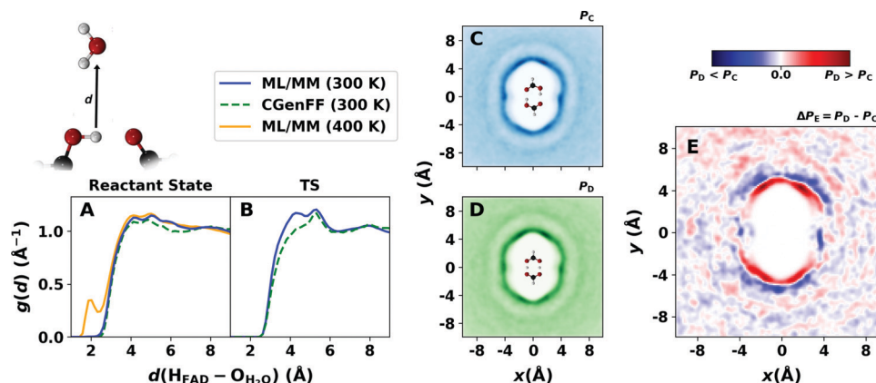
Fig. 6 The radial distribution function g(d) for the water–oxygen atoms around hydrogen atoms \text{H}_A and \text{H}_B of FAD in the reactant (A) and TS (B) structure from the ML/MM (blue line) and CGenFF (dashed green line) simulations at 300 K. Panel (A) also shows g(d) from one entire ML/MM simulation at 400 K (orange line) including formic acid dominantly as cyclic dimer and separated monomers (see Fig. 2A). Panels (C and D) report the solvent distribution functions P(x, y) around FAD from ML/MM MD simulations in its reactant (C) and TS (D) structures, respectively, and panel (E) reports the difference \Delta P(x, y) = P_D - P_C between the two.
