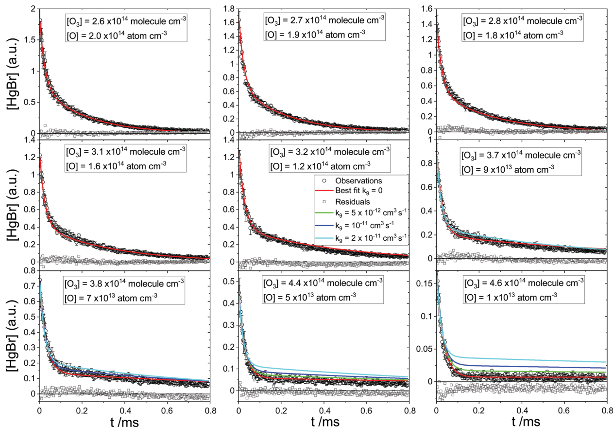
Fig. 7 As Fig. 6 for nine HgBr decays with varying laser energy at constant [O_3]_0 . The green, blue and cyan lines correspond to fit results for k_9 = 5 \times 10^{-11} \text{ cm}^3 \text{ molecule}^{-1} \text{ s}^{-1} , k_9 = 10^{-11} \text{ cm}^3 \text{ molecule}^{-1} \text{ s}^{-1} and k_9 = 2 \times 10^{-11} \text{ cm}^3 \text{ molecule}^{-1} \text{ s}^{-1} , respectively. Green, blue and cyan simulated traces are only shown in those panels where they do not overlap with the red traces. Note that for the bottom right panel the residual is shifted by an arbitrary constant for clarity.
