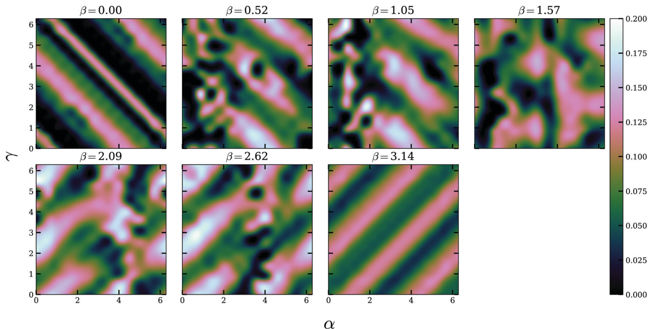
Fig. 4 Value of the fidelity (eqn (17)) optimised for individual orientations of fenchone as a function of the Euler angles \alpha , \beta and \gamma . Lighter areas correspond to higher fidelities, i.e. better chiral distinguishability.
