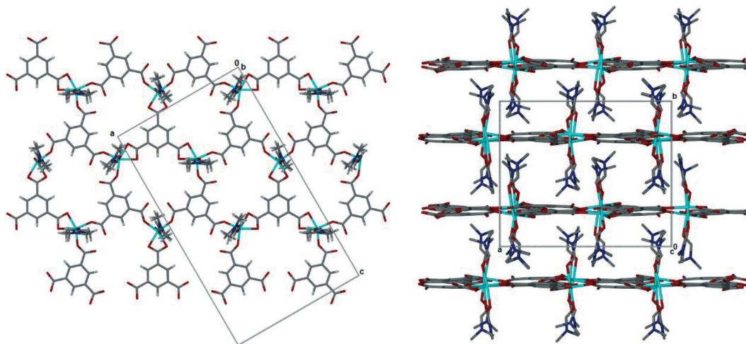
Fig. 2 (Left) The 2D honeycomb layer in 1 , viewed down [010]. Guest DMF omitted. (Right) Interdigitation of 2D layers in 1 , viewed down [001]. Guest DMF and hydrogen atoms omitted for clarity.
