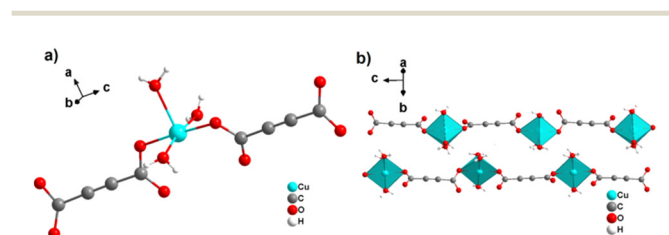
Fig. 14 Crystal structure of copper acetylenedicarboxylate [Cu(ADC)(H 2 O) 3 ](H 2 O) showing: (a) the coordination environment of a Cu 2+ cation and (b) two one-dimensional polymeric chains, which are held together by hydrogen bonding. Graphics redrawn from the cif file (CSD-Refcode MACGAZ). 55
