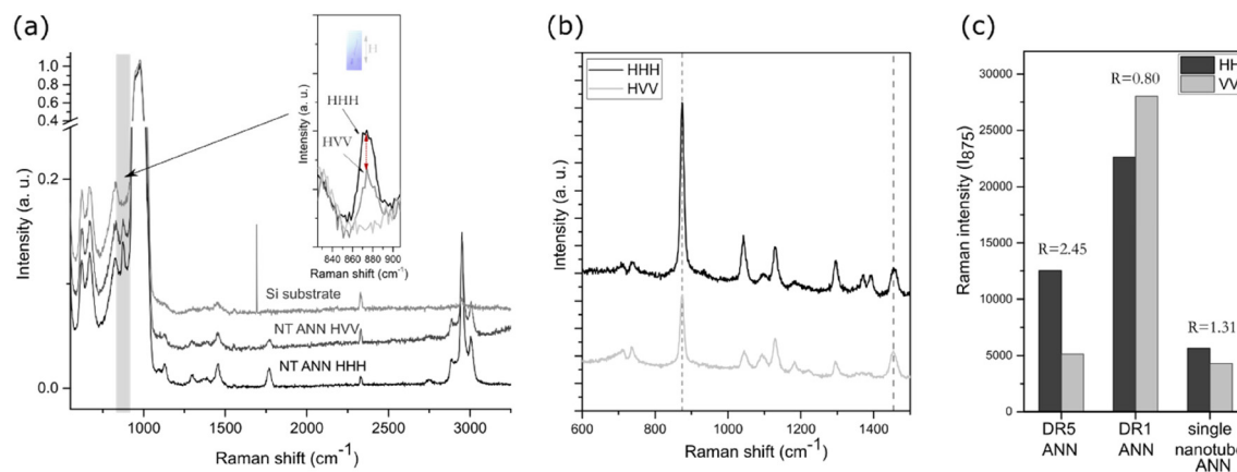
Fig. 4 Polarized Raman spectra of (a) extracted annealed nanotubes in pore length direction (HHH) and perpendicular (HV) for orientation assessment with magnification of 875 cm -1 peak (b) and drawn film in drawing direction (HHH) and perpendicular (VV). (c) Comparison of Raman intensities for horizontal and perpendicular values of 875 cm -1 peak for annealed drawn film (DR5 ANN), non-oriented film (DR1 ANN) and single nanotube, with calculated orientation ratio ( R ) as HHH normalized to VVV values.
