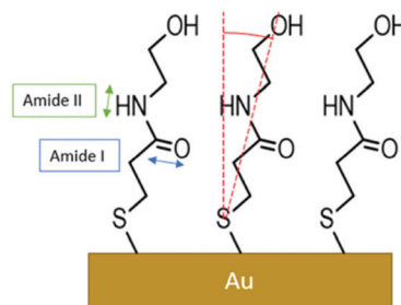
Fig. 7 NMPA SAM on a Au gate structure. Directions of the dipole moments associated with the amide I and amide II signals are indicated with blue and green double arrows, respectively. The red arc indicates the \theta angle between the surface normal and chain direction. The sketch is not in scale and exaggerated to make the orientation more evident.
