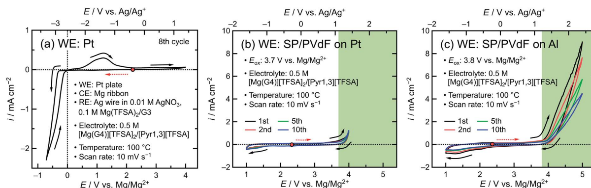
Fig. 2 Cyclic voltammograms of cells featuring a 0.5 M [Mg(G4)][TFSA] 2 /Pyr1,3[TFSA] solution as the electrolyte at 100 °C and a scan rate of 10 mV s -1 . The cells comprised (a) a Pt plate, (b) a blank electrode on a Pt current collector, and (c) a blank electrode on an Al current collector as the working electrodes (WEs); a Mg ribbon as the counter electrode (CE); and a Ag wire in a 0.01 M AgNO 3 , 0.1 M Mg (TFSA) 2 /G3 solution as the reference electrode (RE). The electrolyte was decomposed at potentials higher than the oxidation potential ( E_{ox} ), as indicated by the green areas in (b) and (c). The open circuit potentials and scan directions are illustrated using solid red circles and arrows, respectively. The dotted arrows indicate the initial potential scan direction. Here, G3, G4, TFSA, and Pyr1,3 denote triethyleneglycol dimethyl ether, tetraethylene glycol dimethyl ether, bis(trifluoromethanesulfonyl)amide, and N -methyl- N -propylpyrrolidinium, respectively.
