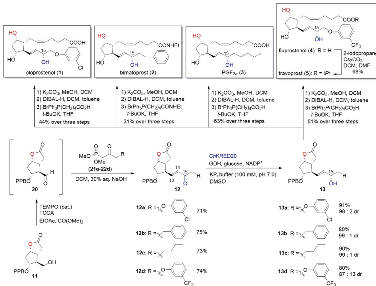
Fig. 5 Completion of the chemoenzymatic total synthesis of cloprostenol (1), bimatoprost (2), PGF_{2\alpha} (3), fluprostenol (4), and travoprost (5).
