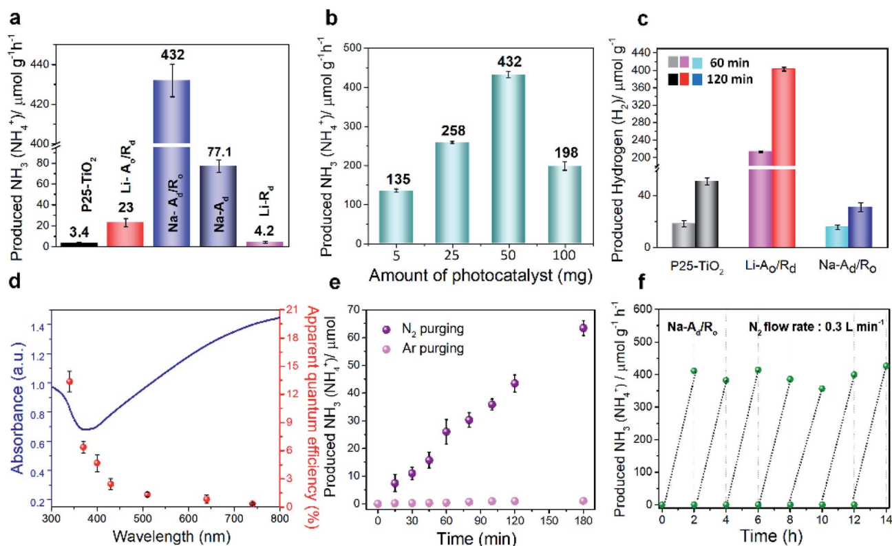
Fig. 3 Photocatalytic N 2 fixation activities of various ordered/disordered TiO 2 samples. (a) The rate of produced NH 3 (NH 4 + ) over P25-TiO 2 , Li-A 0 /R d , Na-A 0 /R o , Li-R d and Na-A d in N 2 saturated water with IPA (14%) as the hole/hydroxyl radical scavenger under solar illumination. (b) The rate of produced NH 3 (NH 4 + ) for Na-A d /R o at various amounts of the catalyst for photocatalytic N 2 reduction. (c) The rate of produced H 2 over P25-TiO 2 , Li-A 0 /R d and Na-A 0 /R o in N 2 saturated-water with IPA (14%) as the hole scavenger under solar illumination. (d) UV-vis diffuse reflectance spectrum (UV-DRS, left axis) and calculated apparent quantum efficiency (AQE, right axis) for N 2 fixation over Na-A d /R o under monochromatic light irradiation. (e) Time-dependent rates of produced NH 3 (NH 4 + ) for Na-A d /R o under N 2 and Ar gas purging. (f) Cycling test of photocatalytic N 2 fixation over Na-A d /R o .
