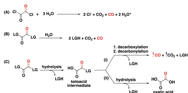
Fig. 2 (A) Decomposition of oxalyl chloride to produce CO. (B) Design of CO donors based on the hydrolysis, decarboxylation, decarbonylation chemistry of oxalyl derivatives. (C) Competing pathways by which 1,2-dicarbonyl CO prodrugs can breakdown in aqueous solution – (i) a CO-generating pathway; (ii) non-CO producing pathway that generates oxalic acid as the product.
