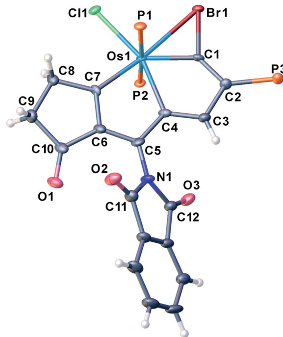
Fig. 4 X-ray crystal structure of the cation of 4a (thermal ellipsoids are set at the 50% probability level and the phenyl groups in the \text{PPh}_3 moieties are omitted for clarity). Selected bond lengths [Å] and angles [°]: Os1–C1: 1.949(5), Os1–C4: 2.146(5), Os1–C7: 2.023(5), Os1–Br1: 2.7241(5), C1–Br1: 1.896(5), C1–C2: 1.366(7), C2–C3: 1.425(7), C3–C4: 1.377(7), C4–C5: 1.414(7), C5–C6: 1.393(7), C6–C7: 1.389(7), C5–N1: 1.379(7), C4–Os1–C1: 68.38(19), C7–Os1–C4: 74.12(19), Os1–C1–Br1: 90.2(2), Br–Os1–C1: 44.10(13), Os1–Br1–C1: 45.67(15).
