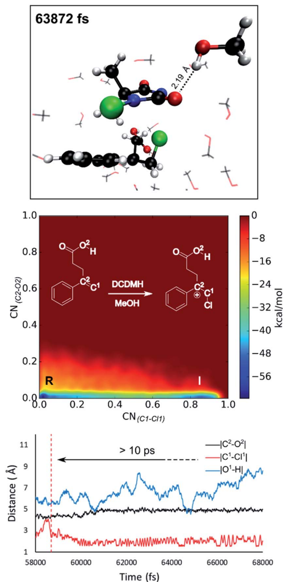
Fig. 5 DCDMH halonium formation of 1a in MeOH. The intermediate phase is stabilized due to the formation of a hydrogen bond between a MeOH molecule and the anionic dechlorinated MCDMH − . This hydrogen bond is visualized for a snapshot of the MtD simulation. No syn -directing interactions are observed between the reactants due to explicit competing interactions with the solvent.
