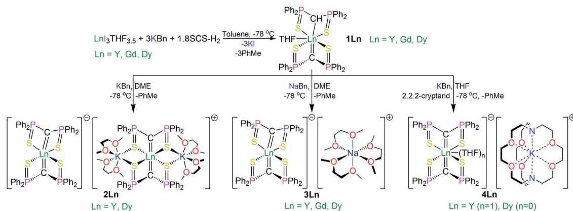
Scheme 1 Synthetic routes to the bis-methanediide complexes 1Ln – 4Ln , Ln = Dy, Y, Gd. The synthesis of 5Dy is very similar, utilising \text{H}_2\text{-C}(\text{PPh}_2\text{NSiMe}_3)_2 instead of \text{H}_2\text{C}(\text{PPh}_2\text{S})_2 and dibenzo-18-crown-6 ether as the auxiliary ligand.
