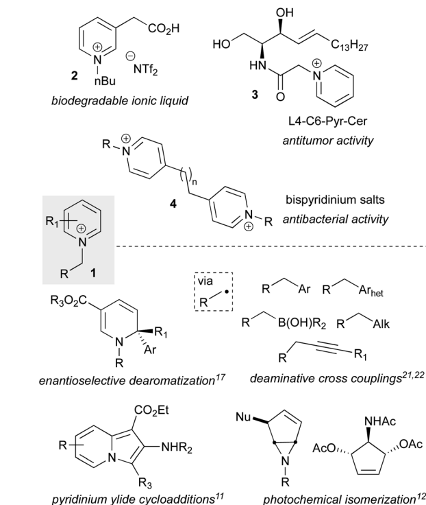
Fig. 1 N-Alkyl pyridinium salts as the active components in materials and bioactive molecules as well as versatile synthetic intermediates.
