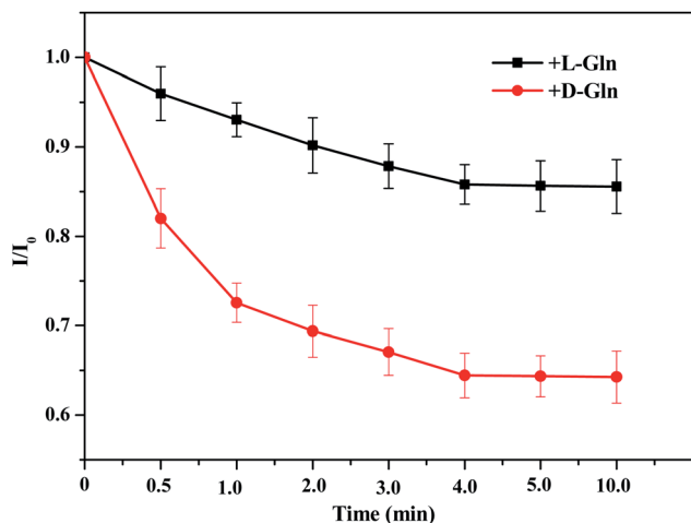
Fig. 11 The effect of incubation time on the I/I_0 of PCN-128Y-1 after adding L-/D-Gln (experimental conditions: 0.05 mg mL -1 MOFs, 50 \mu L 1 mol L -1 L- or D-Gln, and 325 nm excitation wavelength).
