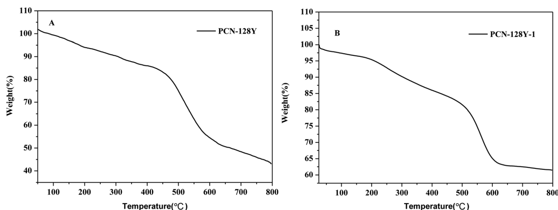
Fig. 6 TG characterization curves of PCN-128Y and PCN-128Y-1.
