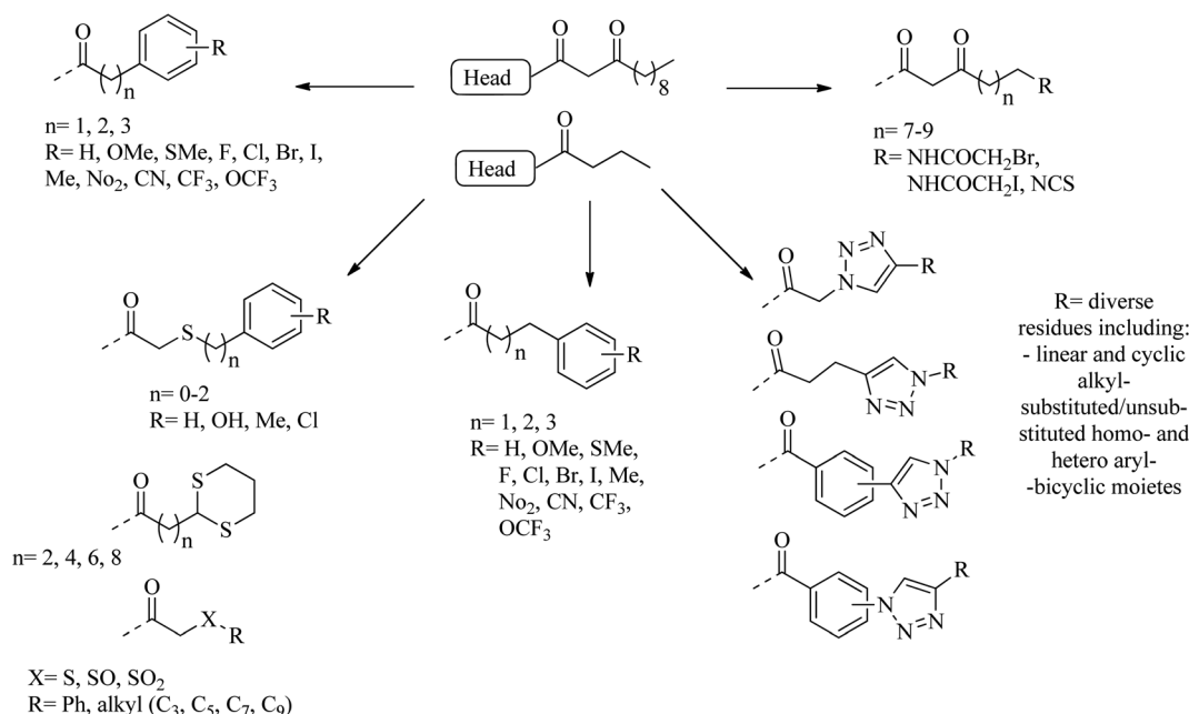
Fig. 13 A diagram of some substituents as tail section replacements to obtain QSL.
