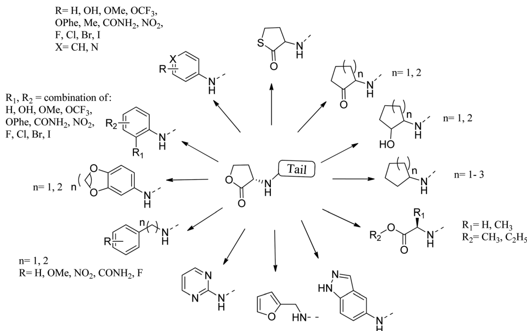
Fig. 12 Some reported substituents as head group replacements in AHL to obtain QSL.
