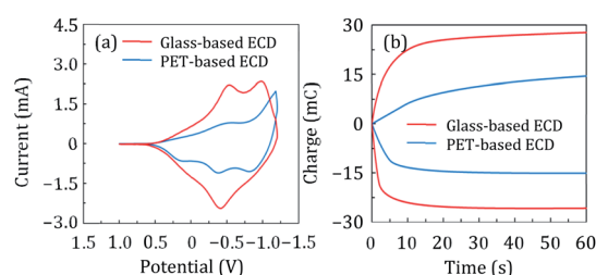
Fig. 3 (a) CV and (b) CC profiles of the glass-based (red) and PET-based (blue) ECDs acquired at a potential scan rate of 5 \text{ mV s}^{-1} .
