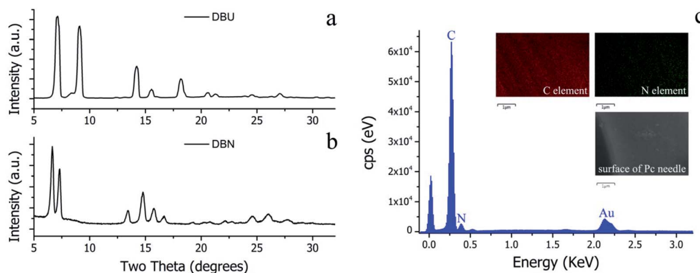
Fig. 4 (a) XRD patterns of H_2Pc crystals from DBU-catalyzed reactions. The matched JCPDS card number is 37-1844. (b) XRD patterns of H_2Pc crystals from DBN-catalyzed reactions. The matched JCPDS card number is 36-1882. (c) Energy-dispersive X-ray (EDX) spectra and elemental scan mapping images of a single H_2Pc needle. The weight percentages (wt%) for C and N elements are 78.34 and 21.66%, and the atomic percentages (at%) for C and N elements are 80.83 and 19.17%, respectively.
