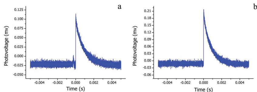
Fig. 8 Transient photovoltage curves of (a) \text{H}_2\text{Pc} needles and (b) \text{H}_2\text{Pc} multiply-laminated crystals.
