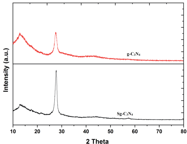
Fig. 2 XRD patterns of g\text{-C}_3\text{N}_4 and \text{Sg-C}_3\text{N}_4 .
