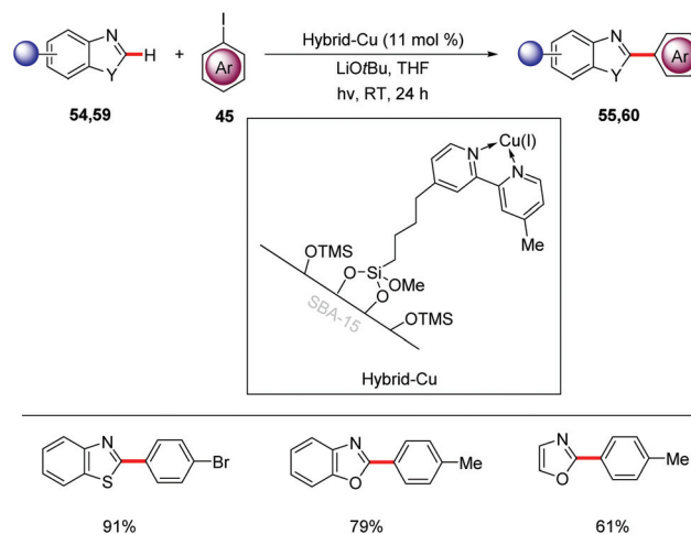
Scheme 20 Heterogenous copper-catalyzed photo-induced C–H arylation.
