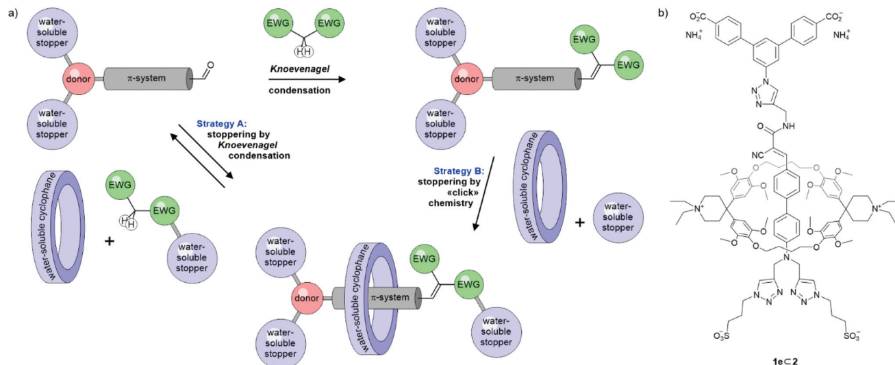
Scheme 1 (a) Both strategies to assemble rotaxanes with a D- \pi -A chromophore as axis considered. (b) Rotaxane 1eC2 obtained via strategy B.
