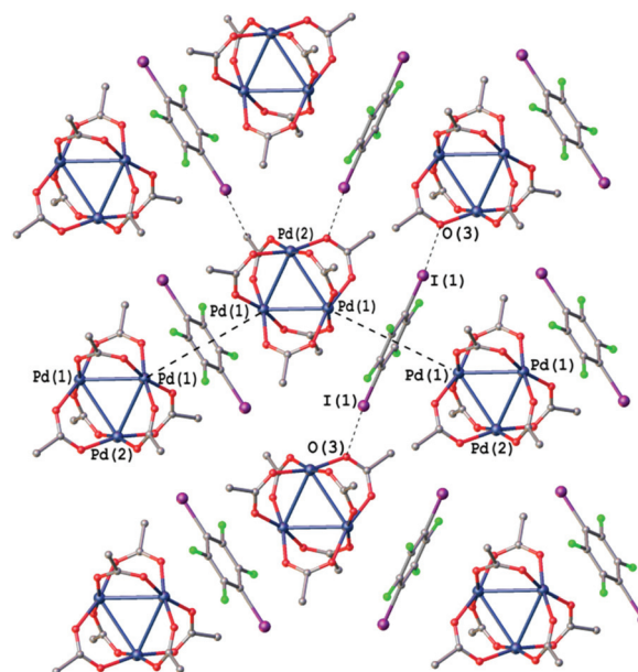
Fig. 8 Crystal structure diagram of [Pd 3 ](1,4-IFB). Selected distances (Å): I(1)...O(3) 3.399, Pd...[Pd 3 ] centroid 3.349. Short I...O contacts and PdO 4 ... \pi interactions are clearly seen in the Hirshfeld surface map (Fig. S5†).
