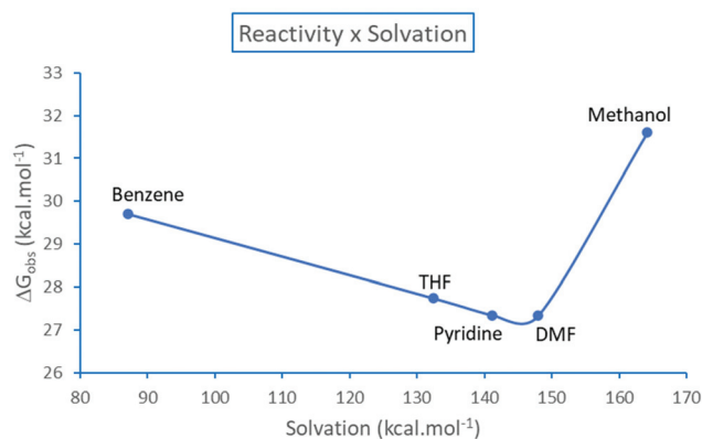
Fig. 5 Observed effective free energy barrier for the TMAF + ArBr reaction as a function of the solvation free energy (absolute values) of the pair of ions N(CH_3)_4^+ + F^- . Theoretical values. 40
