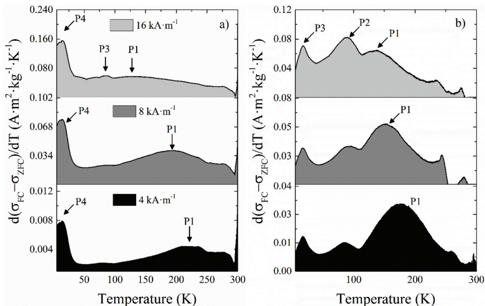
Fig. 5 Differential ZFC magnetization curves with respect to the temperature for samples (a) NO18 and (b) NS18 obtained at external fields of 4, 8 and 16 \text{kA m}^{-1} .
