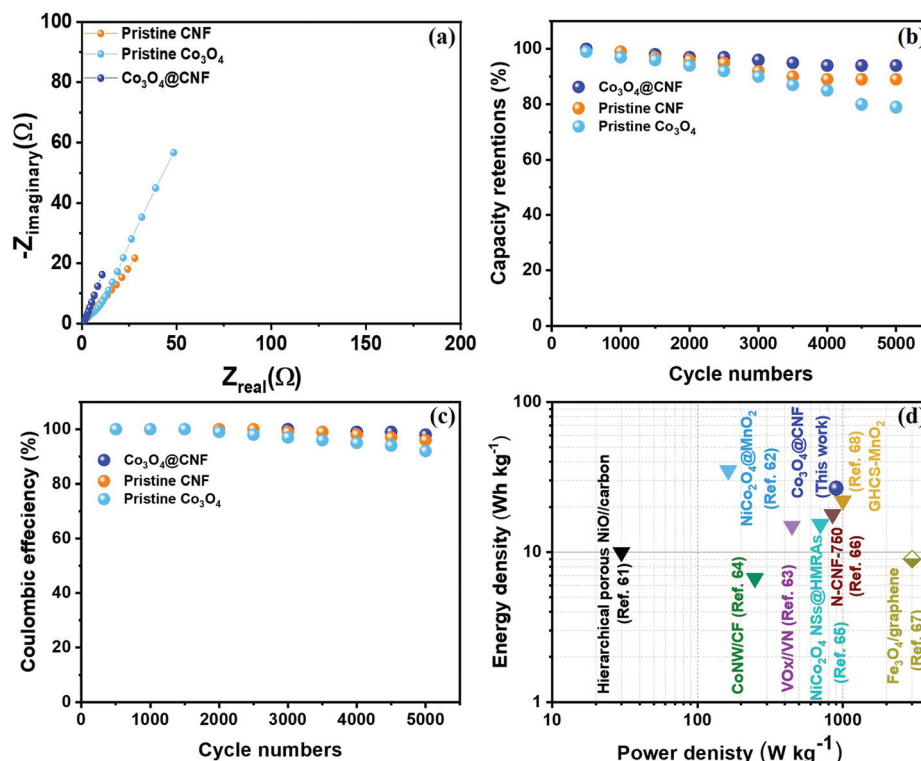
Fig. 7 Electrochemical performance of the SSC devices for the pristine \text{Co}_3\text{O}_4 nanoparticles, pristine CNF and 1D \text{Co}_3\text{O}_4@\text{CNF} hybrid electrodes: (a) EIS plot, (b and c) capacity of retentions and coulombic efficiency of electrodes at 15 \text{ A g}^{-1} of current density over 5000 cycles and (d) Ragone plot.
