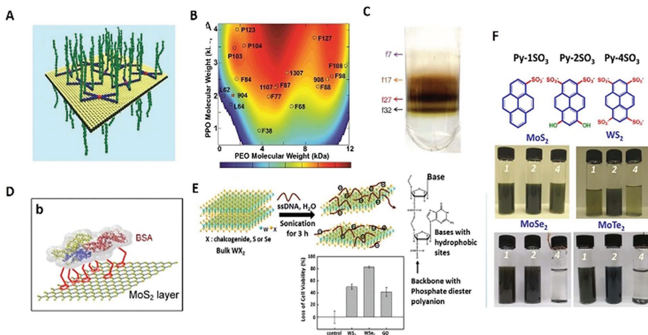
Fig. 6 (A) Schematic for monolayer MoS 2 with tetronic block copolymers absorbed on the surface. (B) MoS 2 concentration map in pluronics and tetronics. (C) Digital picture of a tube with MoS 2 bands after the first iteration of DGU. (D) Schematic diagram of BSA binding with single-layer MoS 2 layer binding. (E) Schematic for ssDNA assisted WS 2 and WSe 2 LPE process. Right: ssDNA backbone structure with phosphate diester polyanion. Bottom: Antibacterial activity comparison of exfoliated WS 2 -ssDNA, WSe 2 -ssDNA and graphene oxide nanosheets against Escherichia coli K-12 MG1655 cells. (F) Four different TMDs exfoliated dispersions with pyrene derivatives. In the digital images 1, 2 and 4 corresponding to the added molecule are Py-1SO 3 (PS1), Py-2SO 3 (Py2) and Py-4SO 3 (Py4). Reproduced from ref. 101, 139, 143, 160 and 161 with permission from IOP Publishing, Wiley-VCH, Springer Nature and the American Chemical Society.
