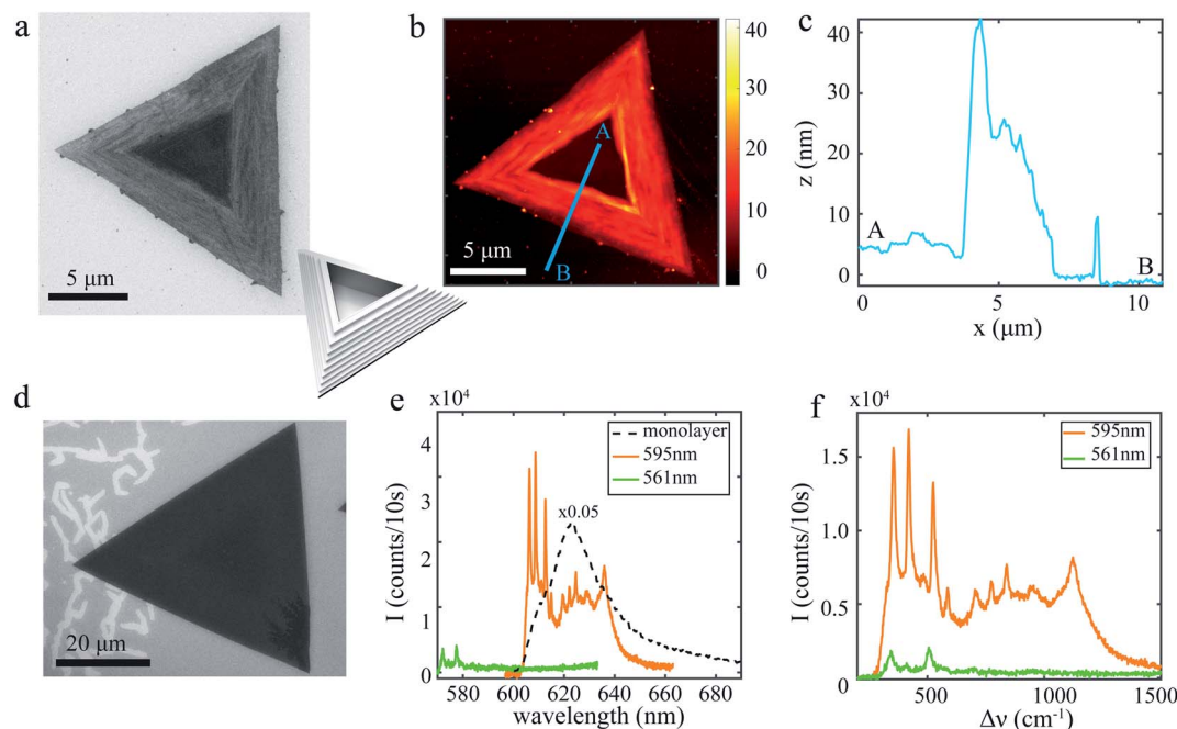
Fig. 1 Hollow WS 2 pyramids. (a) SEM image of the hollow WS 2 pyramid. The lines along the sides indicate the single stair steps, whereas the darker region in the middle is the crater. (Inset) Schematic representation of the hollow pyramid. (b) AFM image of the hollow WS 2 pyramid. The blue line indicates the position of the AFM crosscut depicted in (c), ranging from A the pyramid crater to B the substrate. (d) SEM image of a WS 2 monolayer on the same substrate. (e) Photoluminescence spectrum of the WS 2 monolayer (black dotted line), and spectra of a pyramid obtained with a 595 nm excitation (orange) and a 561 nm excitation (green). When converting the x-axis to wavenumber \Delta\nu in (f), the spectral response on the two different lasers overlaps nicely, indicating that the collected light originates from Raman processes rather than photoluminescence.
