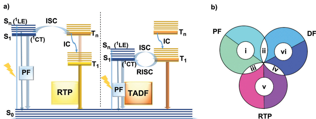
Fig. 1 (a) Jablonski diagram, presenting an overview of photoabsorption, prompt fluorescence (PF), thermally activated delayed fluorescence (TADF) and room temperature phosphorescence (RTP). ISC – intersystem crossing; RISC – reverse intersystem crossing; IC – internal conversion; (b) combinations of DE.
