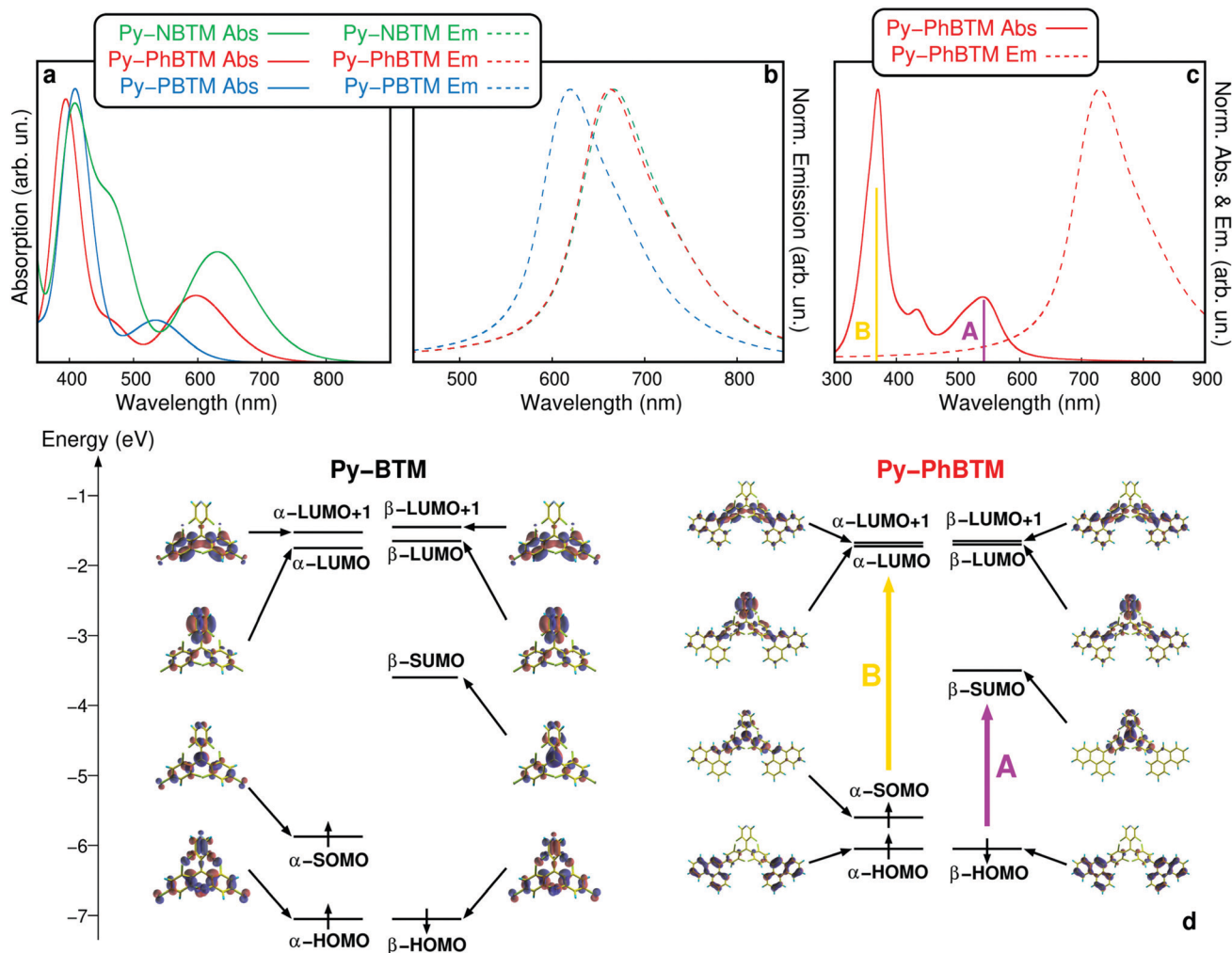
Fig. 4 TDDFT absorption (a) and normalized emission (b) spectra of PyNTBM (green), PyPhBTM (red) and PyPBTM (blue). (c) Normalized TDDFT vibronic absorption and emission spectra of PyPhBTM ; a solvatochromic shift has been applied, as discussed in the text. (d) Unrestricted Kohn–Sham molecular orbitals calculated in the case of PyBTM (left) and PyPhBTM (right). The two main transitions in the visible and near-UV regions of the PyPhBTM spectrum (A and B, respectively) have been highlighted in panel (c) and their main contributions in terms of single-particle excitation have been indicated in panel (d).
