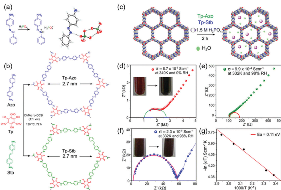
Fig. 19 COFs as proton conductors using azo-moiety. (a) Protonation of azo N-atom by H_3PO_4 (PA). (b) Design and synthesis of COFs. (c) Doping of H_3PO_4 doping in COFs. (d) Proton conductivity of PA@Tp-Azo at 0% relative humidity at 340 K. (e) Proton conductivity of PA@Tp-Azo at 98% relative humidity at 332 K. (f) Proton conductivity of PA@Tp-Stb at 98% RH at 332 K. (g) Calculation of activation energy ( E_a ) for PA@Tp-Azo in hydrous conditions by the methods of Arrhenius. Reproduced with permission. 100 Copyright 2014, American Chemical Society.
