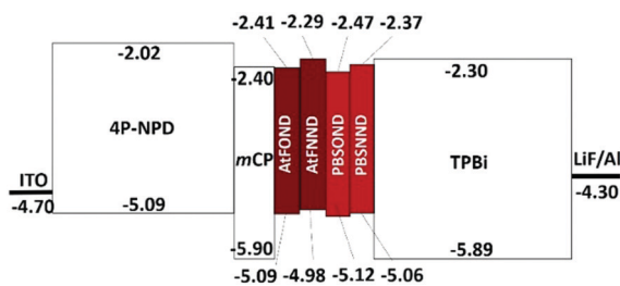
Fig. 7 Energy level (eV) alignment of materials involved in the NIR OLEDs.
