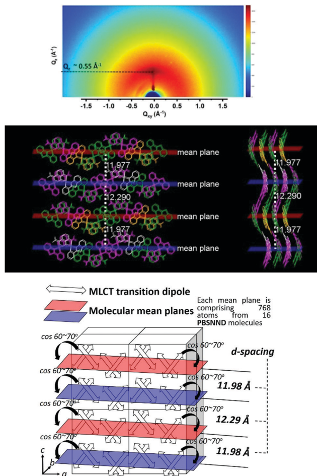
Fig. 11 Top: 2D-GIWAXS patterns for a vacuum-deposited thin film of PBSNND. Centre: Molecular array in the crystal structure of PBSNND with a \sim 90^\circ difference of two viewing angles. Bottom: The schematic display of the centre picture with the labels of MLCT transition dipole, molecular mean plane, and d -spacing.
