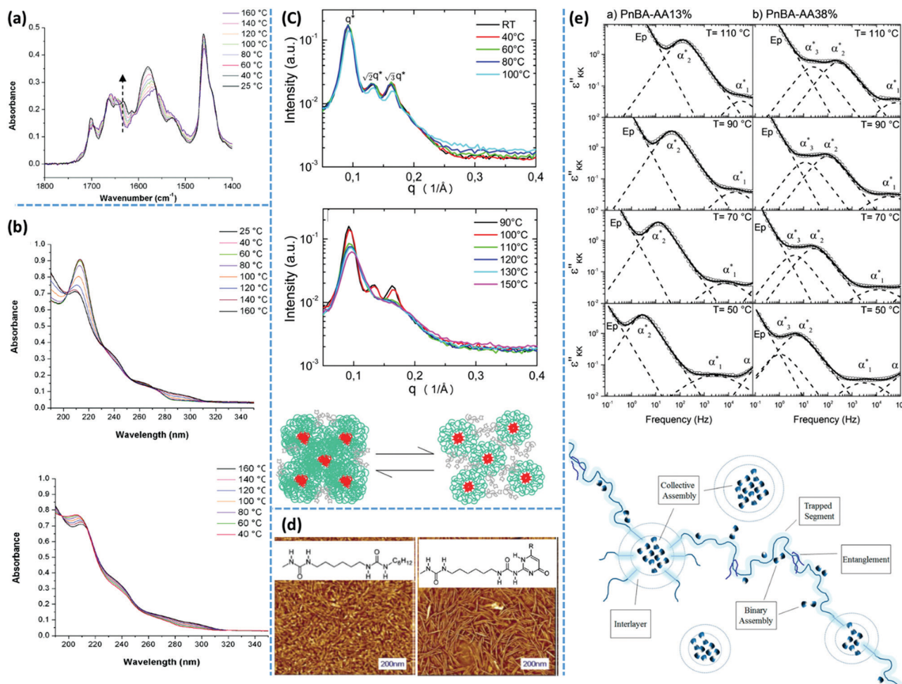
Fig. 5 Representative applications of different characterization techniques for evaluation of supramolecular polymer networks subject to stacking of their associative groups: (a) temperature-variable infrared spectroscopy and (b) UV-vis spectroscopy of telechelic PEB functionalized with UPy groups. 100 (c) SAXS spectra of monofunctional PIB with 2,6-diaminotriazine motifs and the corresponding proposed morphology. 40 (d) AFM image of UPy-functionalized PEB demonstrates nanofibers while that of urea-functionalized does not. 87 (e) Dielectric spectroscopy of PnBA functionalized with AA groups and the proposed general picture of the morphology. 60 Panels (a and b), (c, d, and e) reprinted from ref. 100, 40, 87 and 60, respectively. Copyright 2011, 2014, 2006, and 2016, American Chemical Society.
