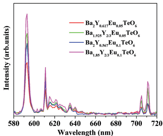
Fig. 9 A comparison of the PL spectra of A- and B-site substituted \text{Ba}_2\text{Y}_{2/3}\text{TeO}_6:\text{Eu}^{3+} .
