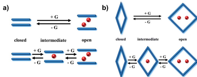
Fig. 4 Schematic illustration of the types of structural transformations in (a) 2D and (b) 3D switching CNs induced by sorbate/guest molecules (G, red balls). Transformation between closed and open phases typically results in a single-step type F-IV s isotherm (top). Transformation between closed, intermediate (partially open) and fully open phases generally leads to a type F-IV m isotherm (bottom).
