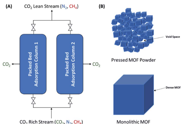
Fig. 1 (A) Schematic of a dual-column pressure swing adsorption/temperature swing adsorption (PSA/TSA) system with MOF packed beds. (B) Representation of the abundant void spaces amongst pressed MOF particles compared with a densified monolithic MOF.
