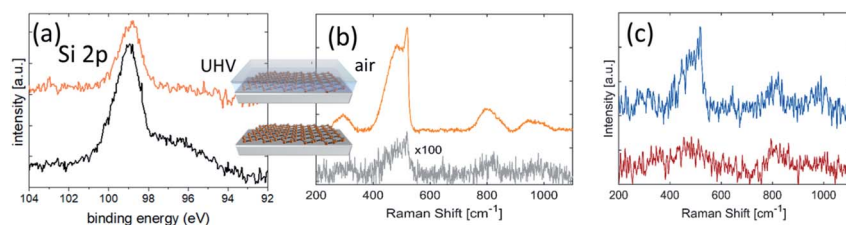
Fig. 2 (a) Si 2p core-level photoemission lines taken on freshly grown silicene-on-silver (bottom) and after Al_2O_3 encapsulation (top). The right-side feature in the former spectrum is related to Ag 4s photoemission from the substrate, and is no longer detected in the encapsulated silicene owing to the Al_2O_3 layer thickness ( \sim 5 nm); (b) Raman spectra of (top) capped and (bottom) uncapped silicene/Ag(111). In both cases the samples are exposed to air when recording the Raman spectrum and the silicene lattice is preserved only in the case of the encapsulated sample; (c) Raman spectra of unprotected silicene/Ag(111) obtained after 1 minute (top: same as the bottom spectrum in panel (b)) and \sim 5 minutes after air exposure (bottom). The spectra are vertically stacked for clarity.
