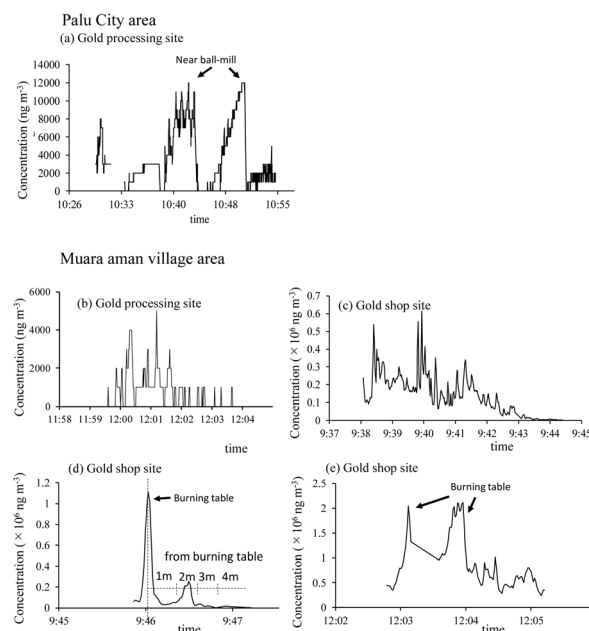
Fig. 3 Fluctuation of GEM concentrations at ASGM sites. Gold shop and gold processing sites. (a) GEM concentration of a gold processing site using the ball mill method in Poboya near Palu (St. 4, Fig. SI1†); (b) GEM concentration of a gold processing site using the ball mill method in Muara Aman; (c–e) Inside Muara Aman gold shops 6 and for (c), GEM concentrations when gold amalgam was not being burned.
