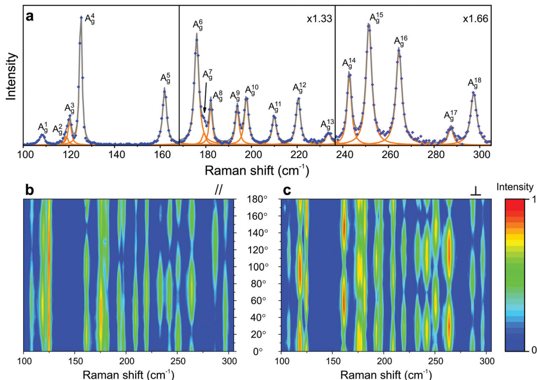
Fig. 7 Characteristic Raman spectrum of the triclinic \text{ReSe}_2 ; (a) Raman spectrum of a monolayer \text{ReSe}_2 showing the 18 A_g modes predicted by group theory. Typical angle-resolved Raman map of \text{ReSe}_2 in the (b) parallel ( \parallel ) and (c) crossed ( \perp ) configurations. The spectra and mapping were collected with a 2.33 eV laser energy. Adapted with permission from ref. 19.
