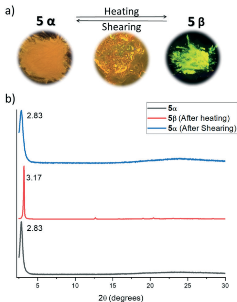
Fig. 7 (a) Photographs of the interconversion between polymorphs 5α and 5β illuminated with a 365 nm lamp. (b) Thermal and subsequent mechanochemical polymorphic transformations followed by powder X-ray diffraction pattern changes.
